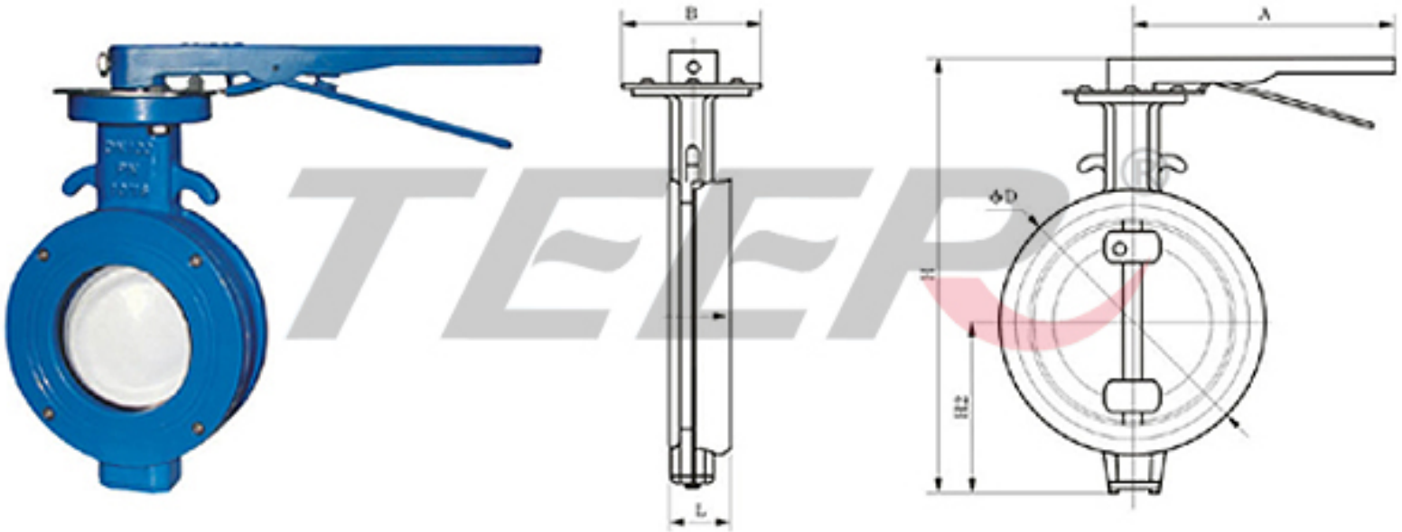
Handle operated butterfly valve
